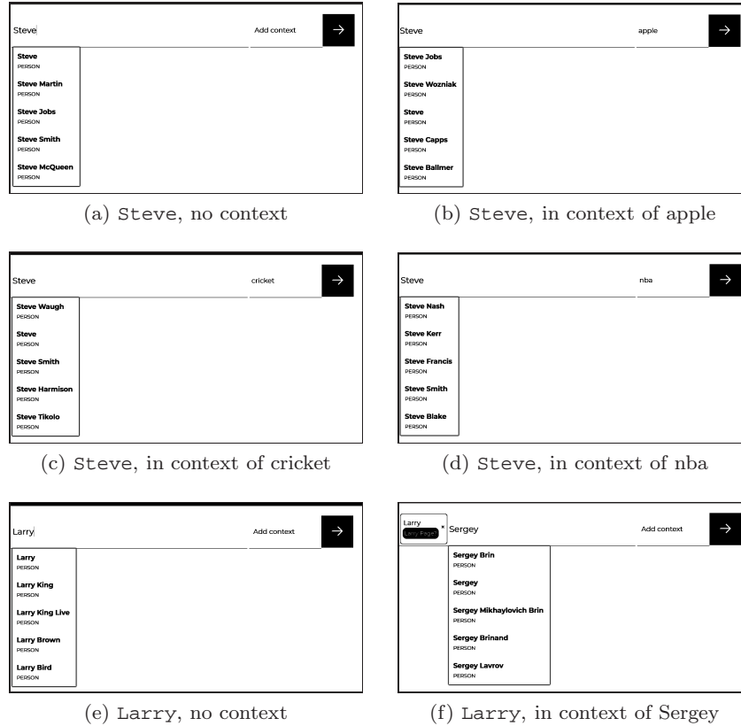
Fig. 3: Some examples of the proposed entity linking approach in action. Note how the suggestions for entities change in sub-figures (a)–(d) with varying contexts. Also note that how the entity context helps retrieve relevant results for larry in sub-figures (e) and (f).
