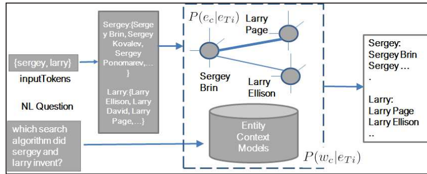
Fig. 2: Illustration of the proposed approach
