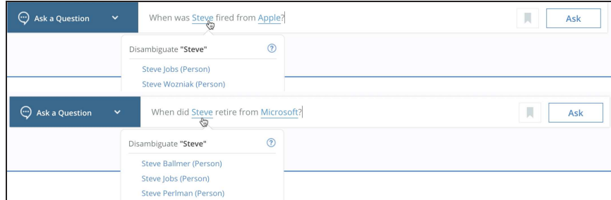
Fig. 1: Entity Suggestions produced by proposed approach using text and entity context in search query.
